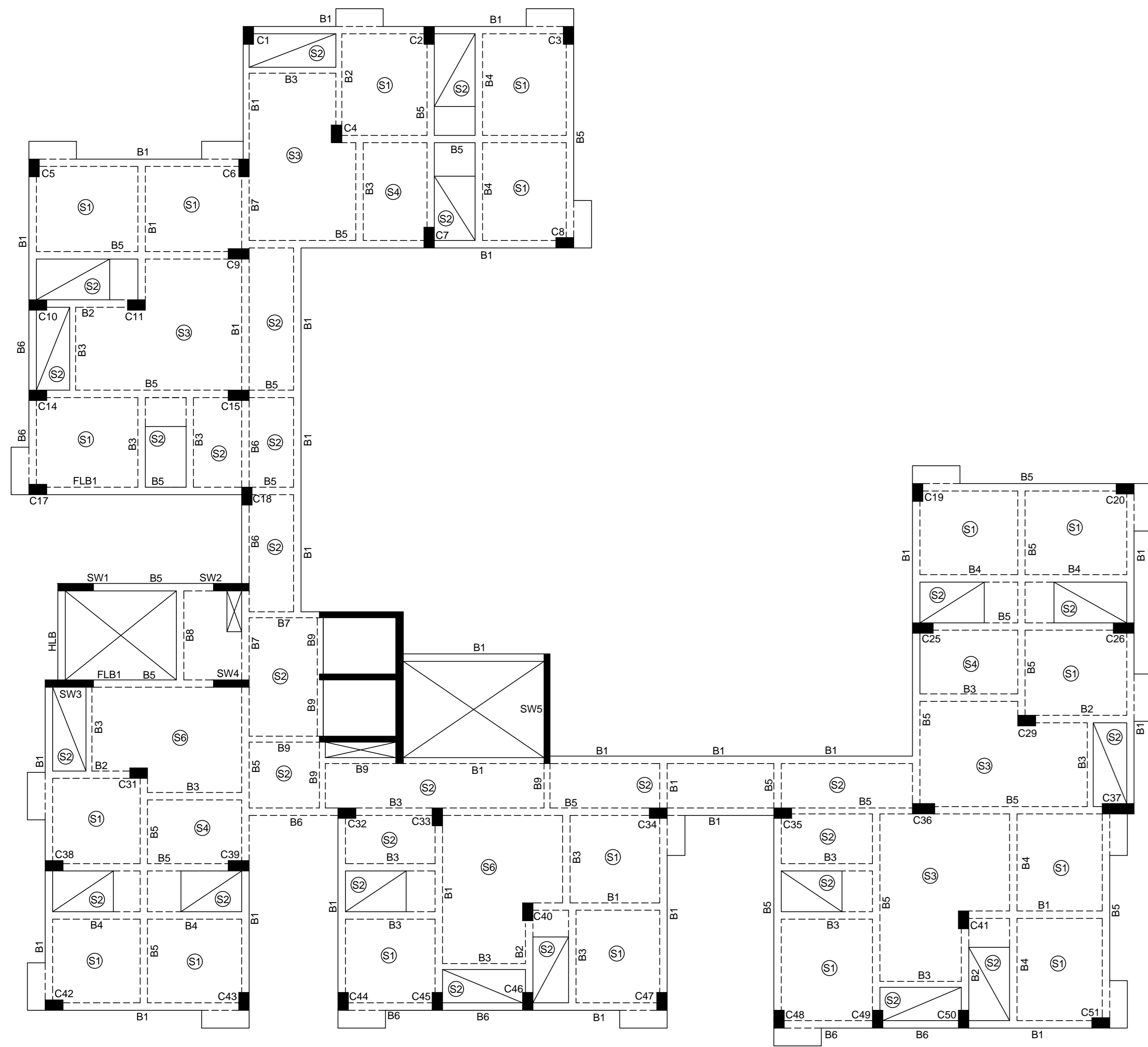
BLOCK-1 ROOF BEAM LAYOUT PLAN.
