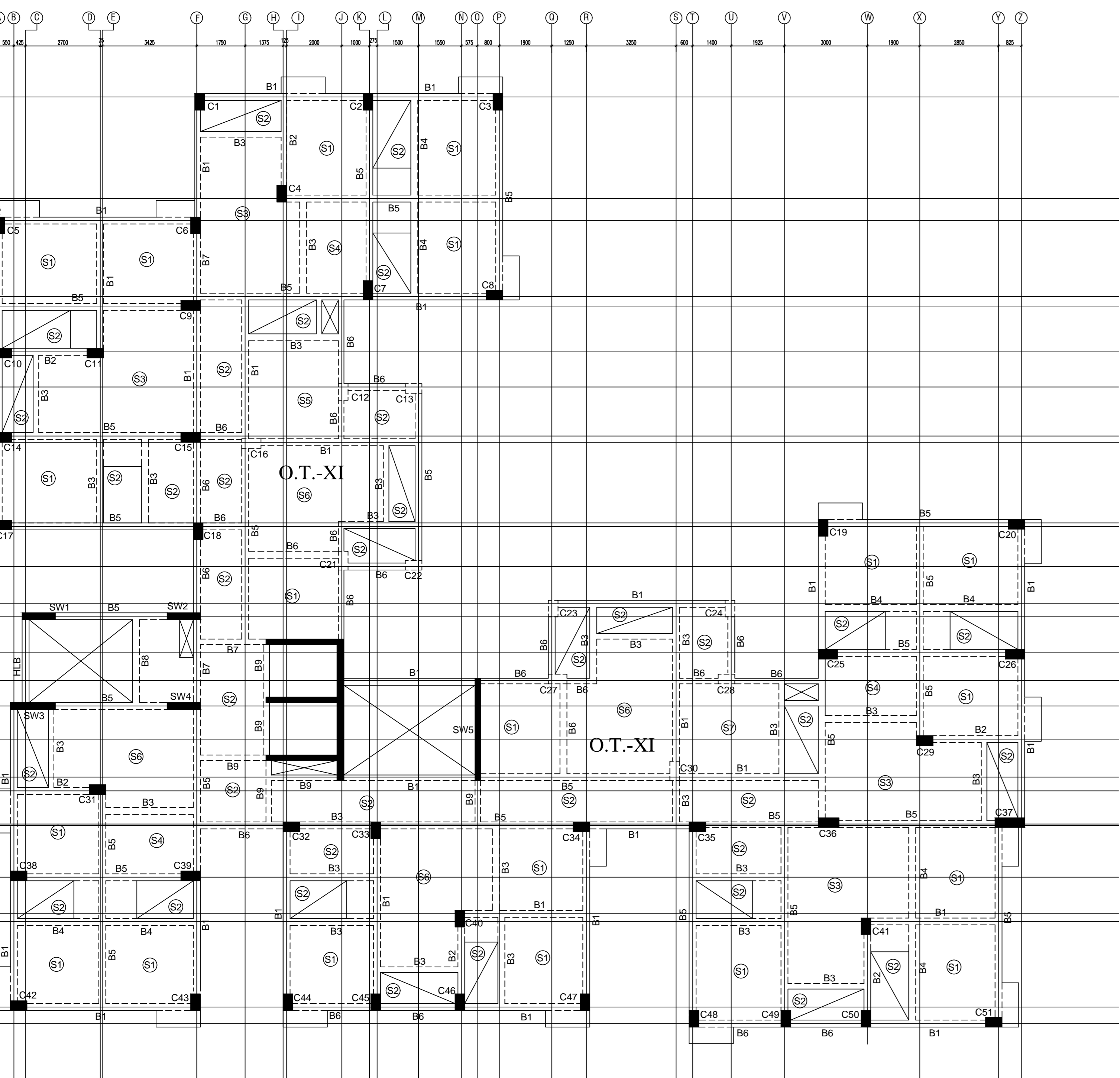
BLOCK-1 10TH ROOF BEAM LAYOUT PLAN.
