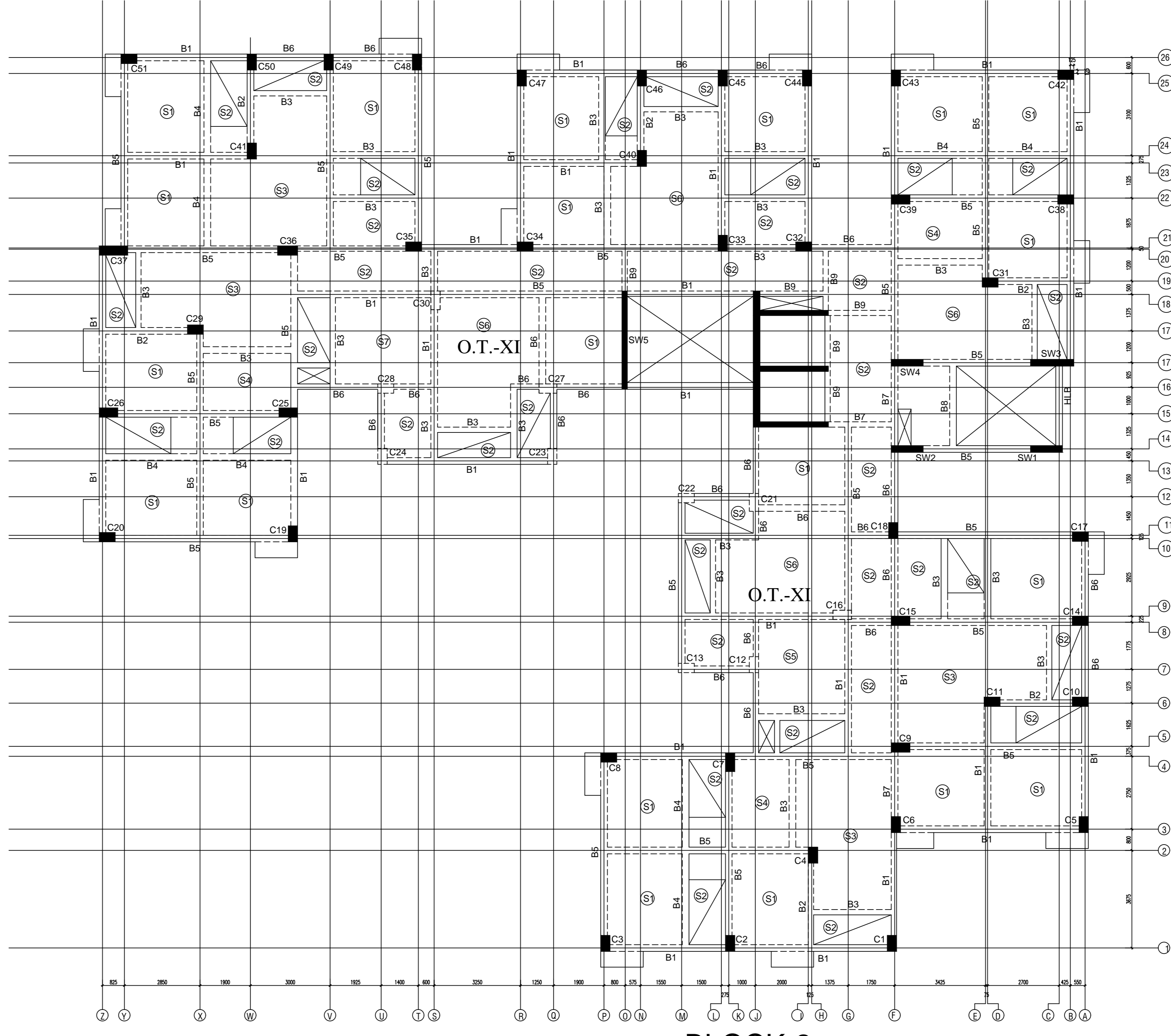
BLOCK-2 10TH ROOF BEAM LAYOUT PLAN.
