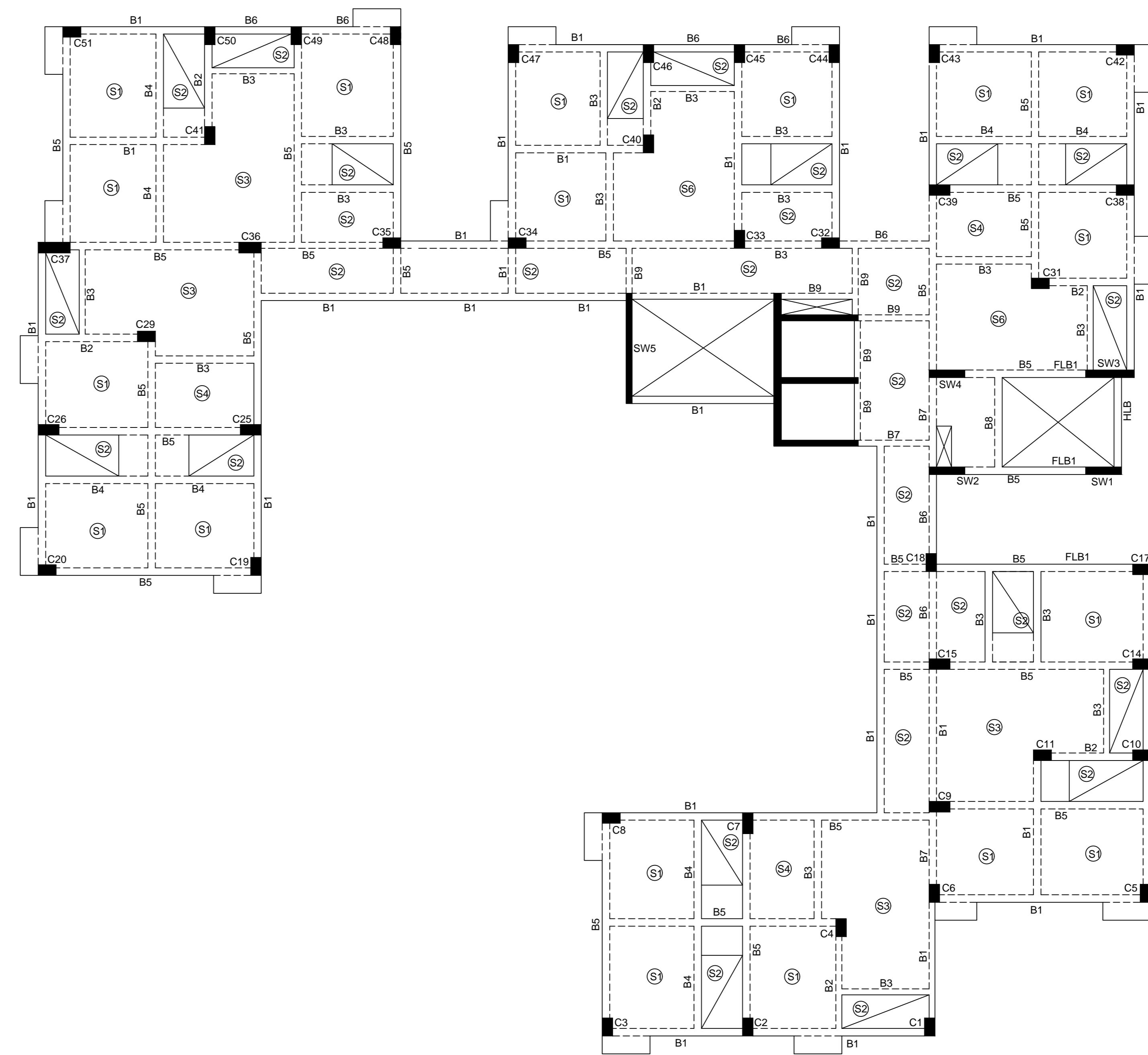
BLOCK-2 ROOF BEAM LAYOUT PLAN.
